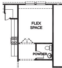
OPTIONAL POWDER ROOM
