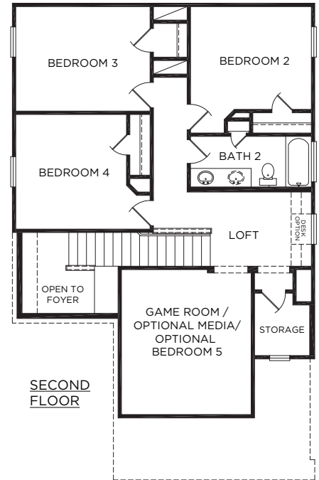
OPTIONAL MEDIA ROOM
